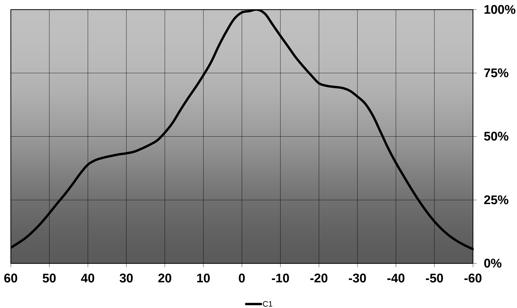
Relative intensity of FP11429_LISA2-WWW-PIN_(SFH_4170S)
